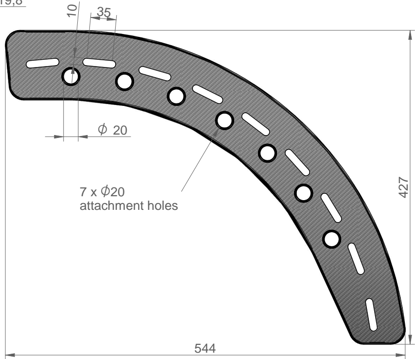
Clewboard Type 5
